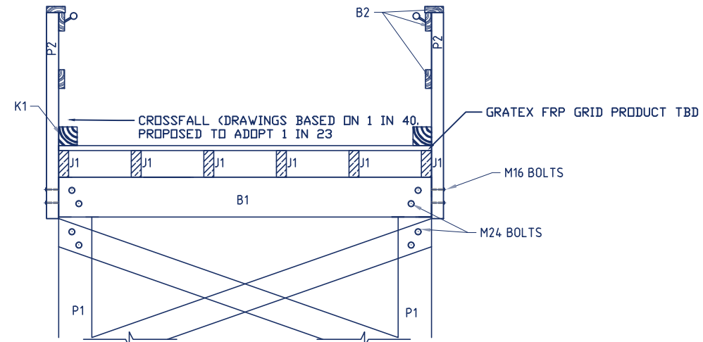
TYPICAL SECTION
