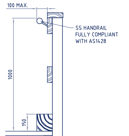
HANDRAIL DETAIL
