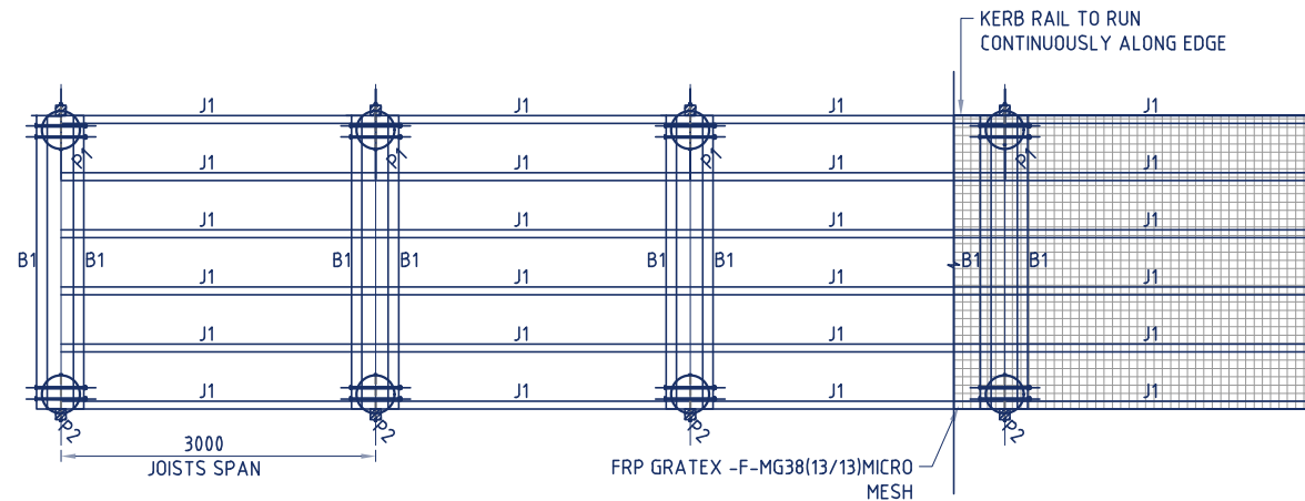
TYPICAL FRAMING PLAN (CURVED SECTIONS NOT SHOWN)
