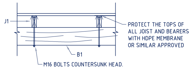
JOIST TO BEARER CONNECTION
