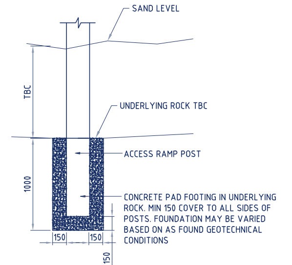
TYPICAL FOUNDATION DETAIL
