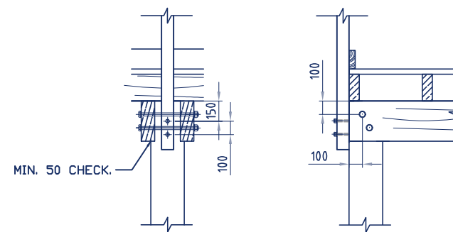
HEADSTOCK TO POST CONNECTION
